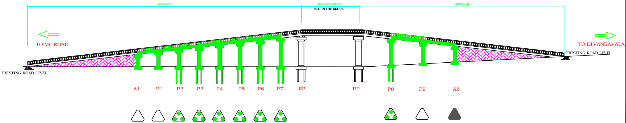
PILE FOUNDATION
